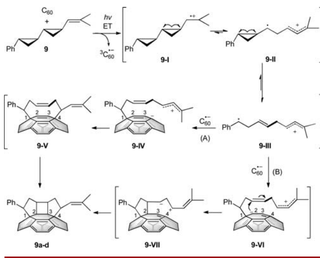
Scheme 3. Proposed Mechanism for the Cycloaddition of 9 and C_{60} , under PET Conditions
