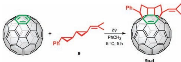
Scheme 2. Reaction of 9 with C 60 in Toluene
